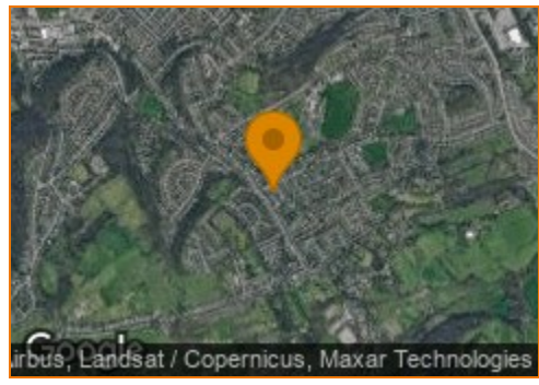
Hybrid Map
